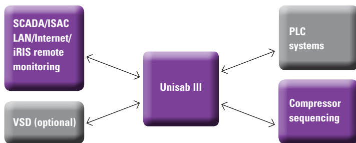
How Unisab III connects to other control equipment
